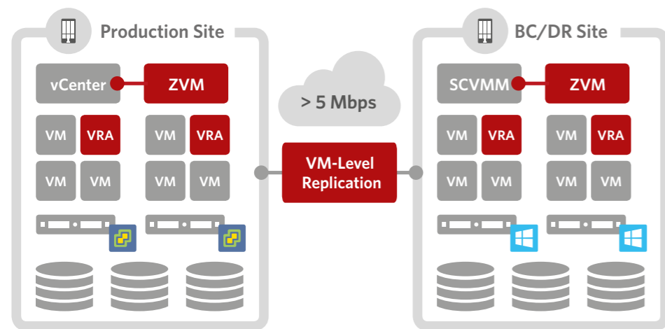
Figure 5. Zerto's Architecture
